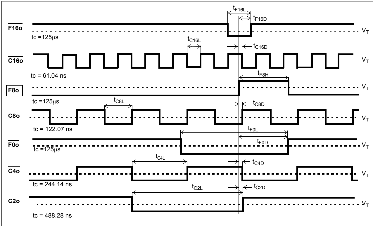
Figure 15 - ST-BUS and GCI Output Timing
